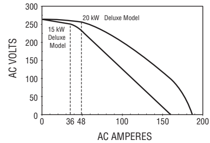
3-PHASE GENERATOR POWER CURVE
