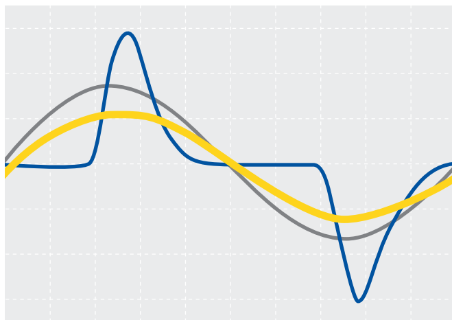
— INPUT VOLTAGE — INPUT CURRENT WITH PFC — INPUT CURRENT WITHOUT PFC
